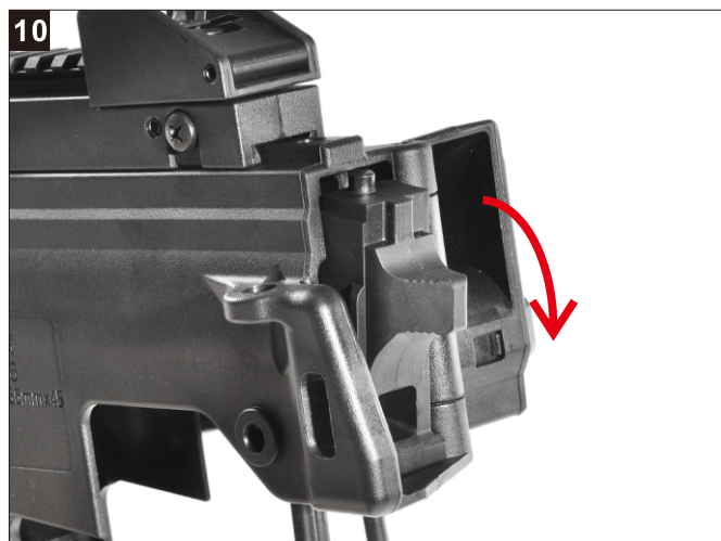
向下扳動複進簧連桿以解除固定。 Push downward to release the Recoil Spring & Guide Rod.
